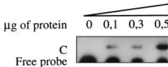
Fig. 1. DNA-binding ability of AlcR(1–60) to a specific half-site. Binding reactions were performed with 32 fmol of a 25-oligonucleotide of the following sequence: 5'-GCCCTCGTGCGGATCCG-TATGCATC-3' and increasing concentrations of protein, 0.1, 0.3 and 0.5 μg of AlcR(1–60) corresponding to 13, 39 and 65 pmol, respectively.
